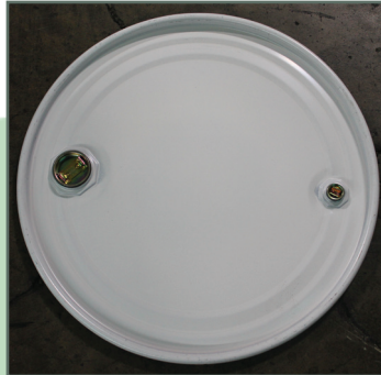
Double Re-enforced Ring Cover w/ 2 x 3/4" flanges and plugs
